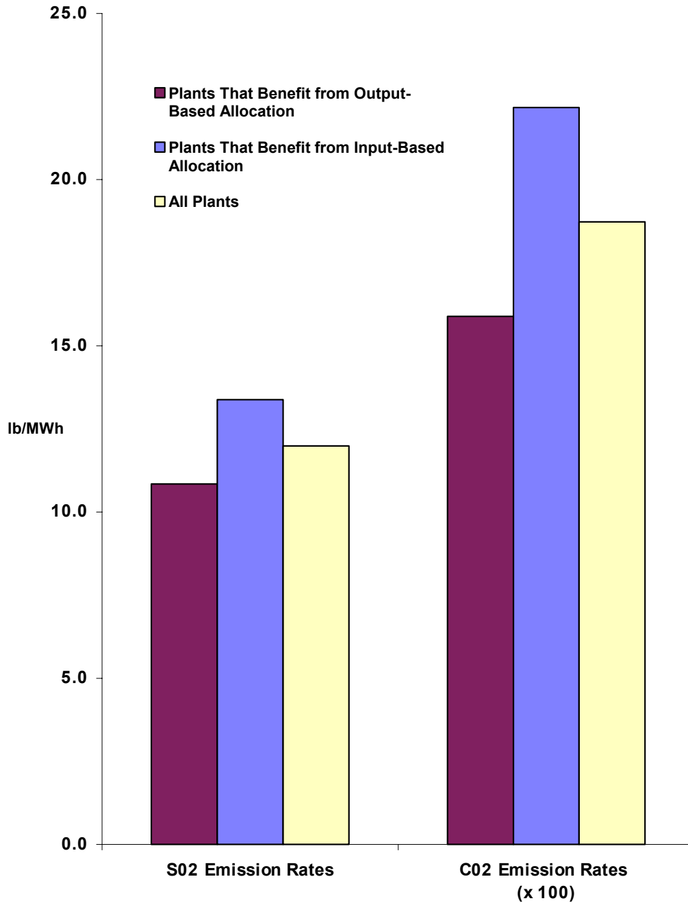
Weighted Average Emission Rates of OTC-Region Plants -- 1998 Actual Data Sorted by Impact of NOx Cap Allocation Method
