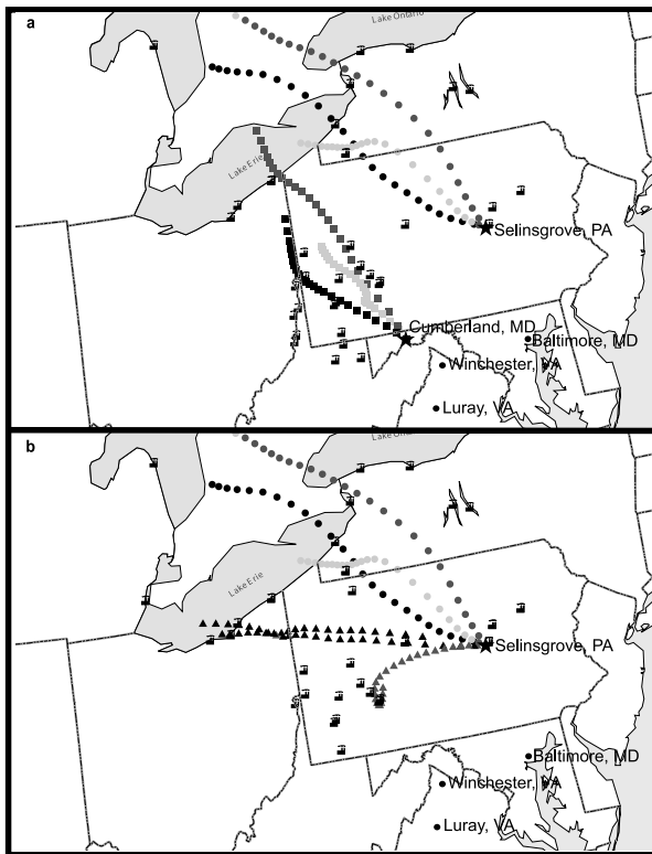
Figure 3. Map of northeastern U.S. showing modeled back trajectories (24 h) from Cumberland, MD and Selingsgrove, PA on 15 Aug, 2003 at 1500 and 2000 UTC, respectively (a); and Selingsgrove, PA on 15 Aug, 2003 (circles) and on 4 Aug, 2002 (triangles) at 2000 and 2100 UTC, respectively (b). Light gray represents 0–500 m, dark gray 500–1500 m, and black 1500–2500 m AGL. Icons represent power plants that fall within trajectory buffers regardless of size or extent of down scaling during the blackout.
