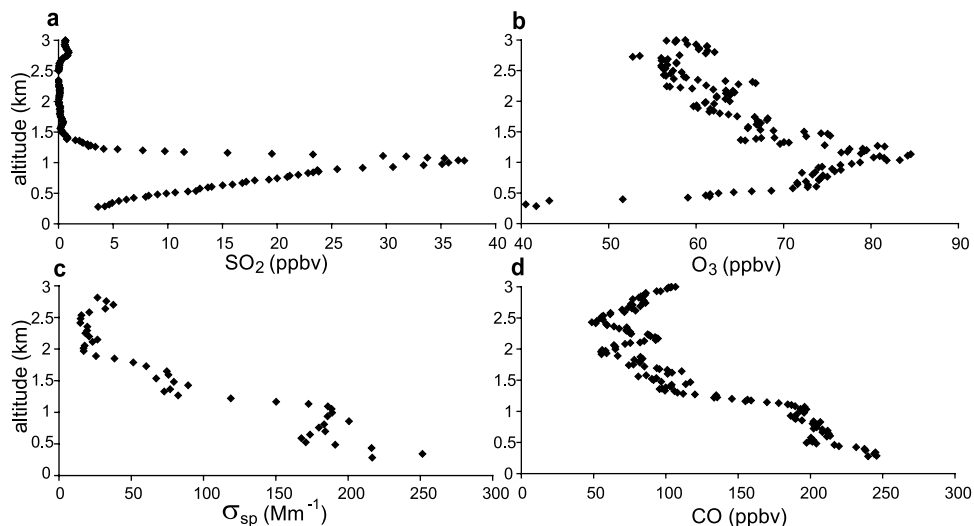
Figure 1. Running 1 min mean SO 2 mixing ratios (a); 10 s O 3 mixing ratios (b); particle light scattering at 550 nm (c); and running 1 min mean CO mixing ratios (d) over Luray, Virginia (outside blackout area) at 1400 UTC (10:00 LST) 15 Aug, 2003.
