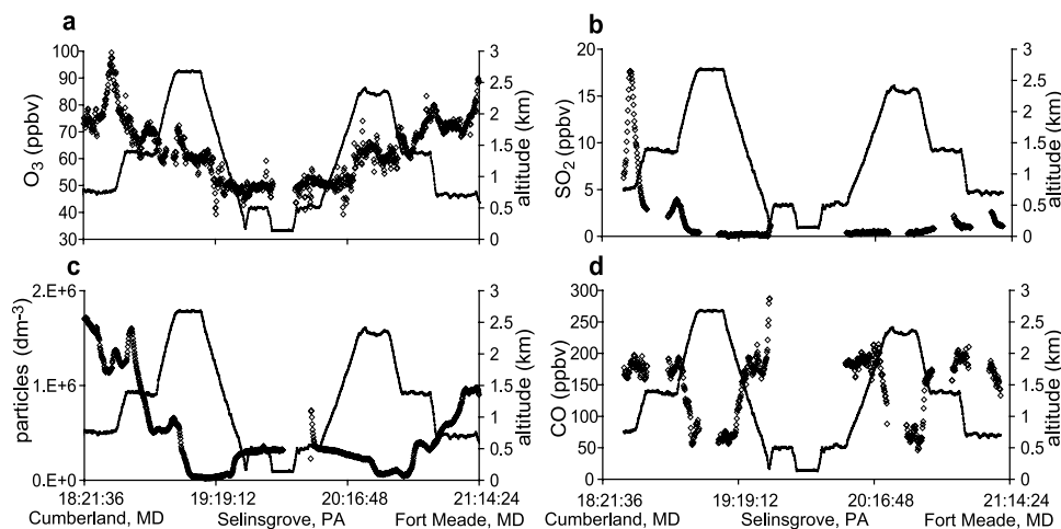
Figure 2. Second flight on August 15, 2003 showing altitude (solid black lines), time (UTC), as well as takeoff, landing and spiral locations. Open diamonds represent 10 s O 3 mixing ratios (a); running 1 min mean SO 2 mixing ratios (b); sub-micrometer particle counts (c); and running 1 min mean CO mixing ratios (d).
