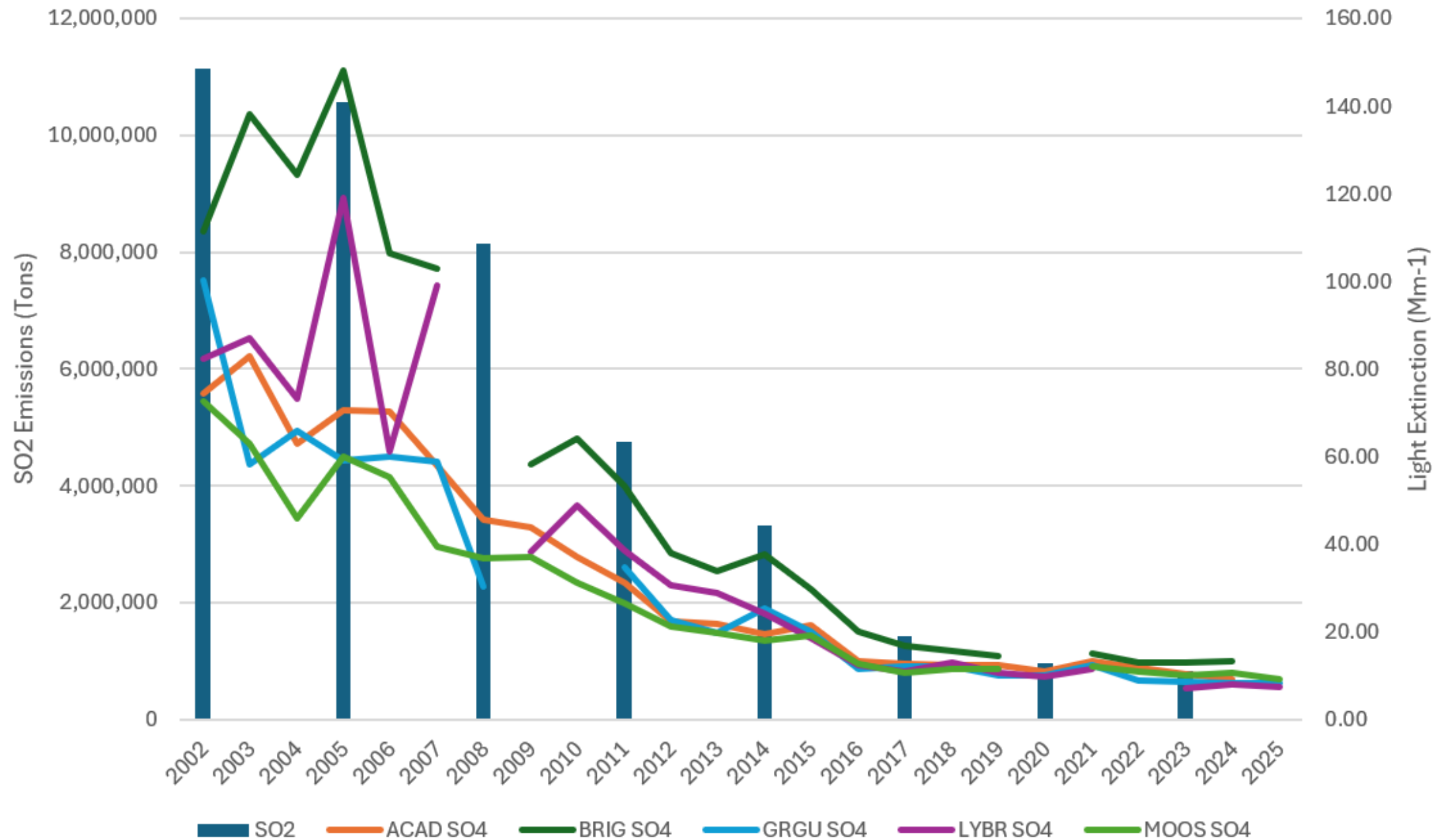
SO2 Emissions and Sulfate Light Extinction
