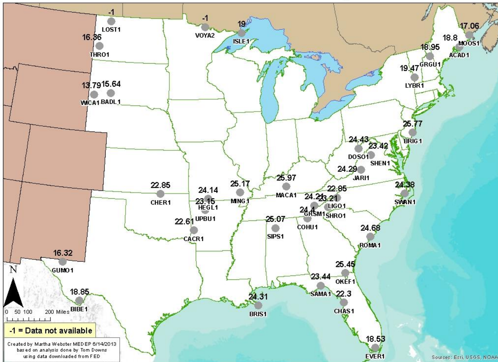
FIGURE E-5: 2011 Annual Deciview for Worst 20% Days
