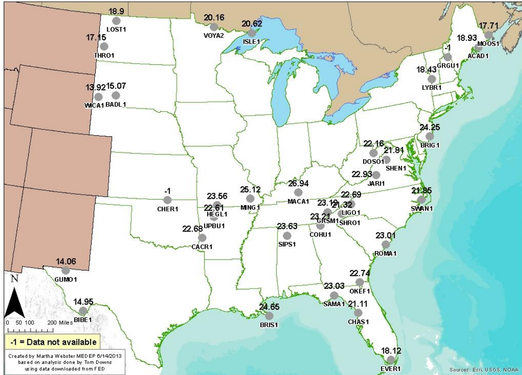
FIGURE E-3: 2009 Annual Deciview for Worst 20% Days
