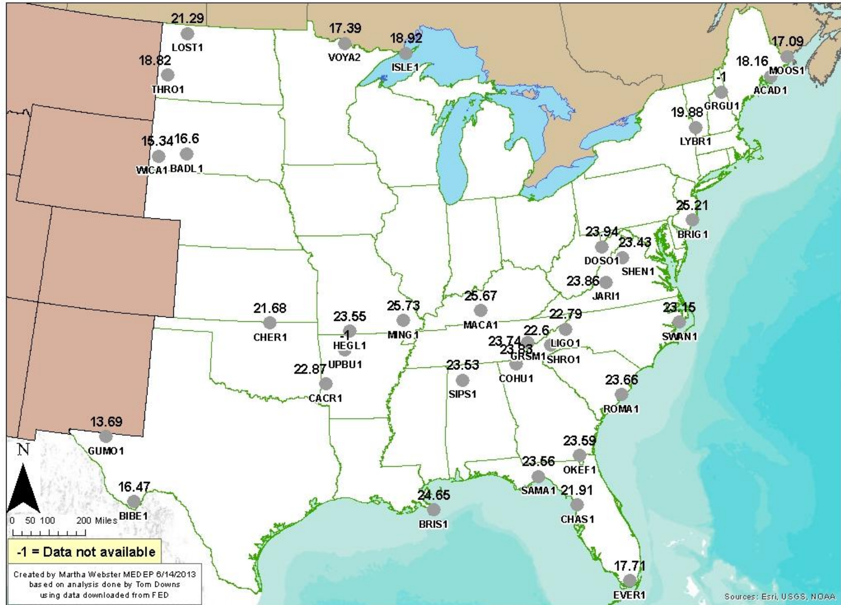
FIGURE E-4: 2010 Annual Deciview for Worst 20% Days
