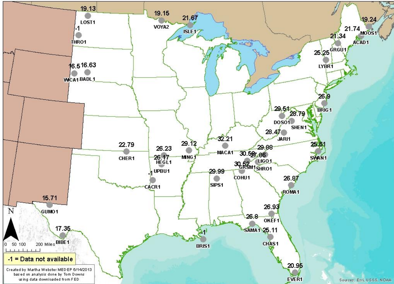
FIGURE E-1: 2007 Annual Deciview for Worst 20% Days
