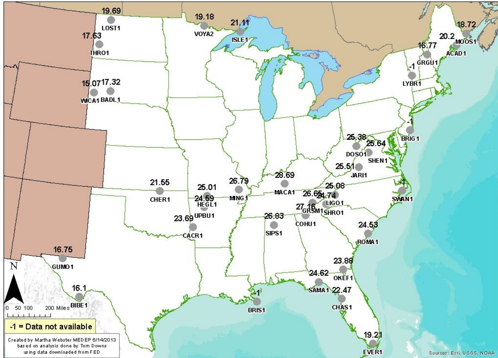
FIGURE E-2: 2008 Annual Deciview for Worst 20% Days
