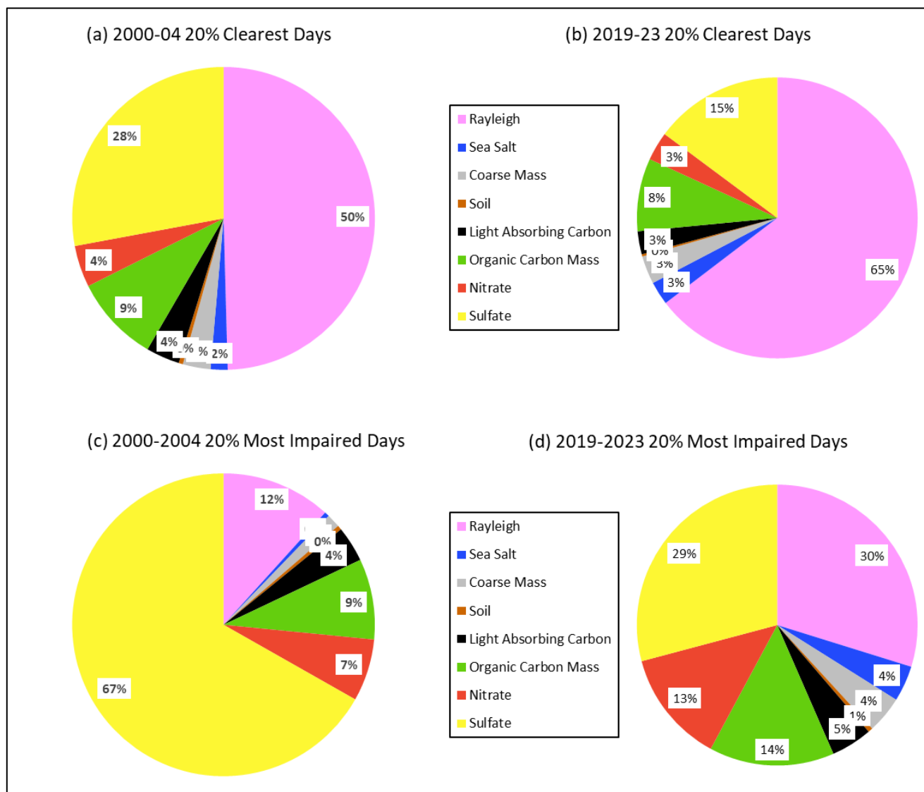
Figure 3-1. Acadia National Park Species Percent Contribution to Baseline (2000-04) and Current (2019-23) Haze Index Levels
