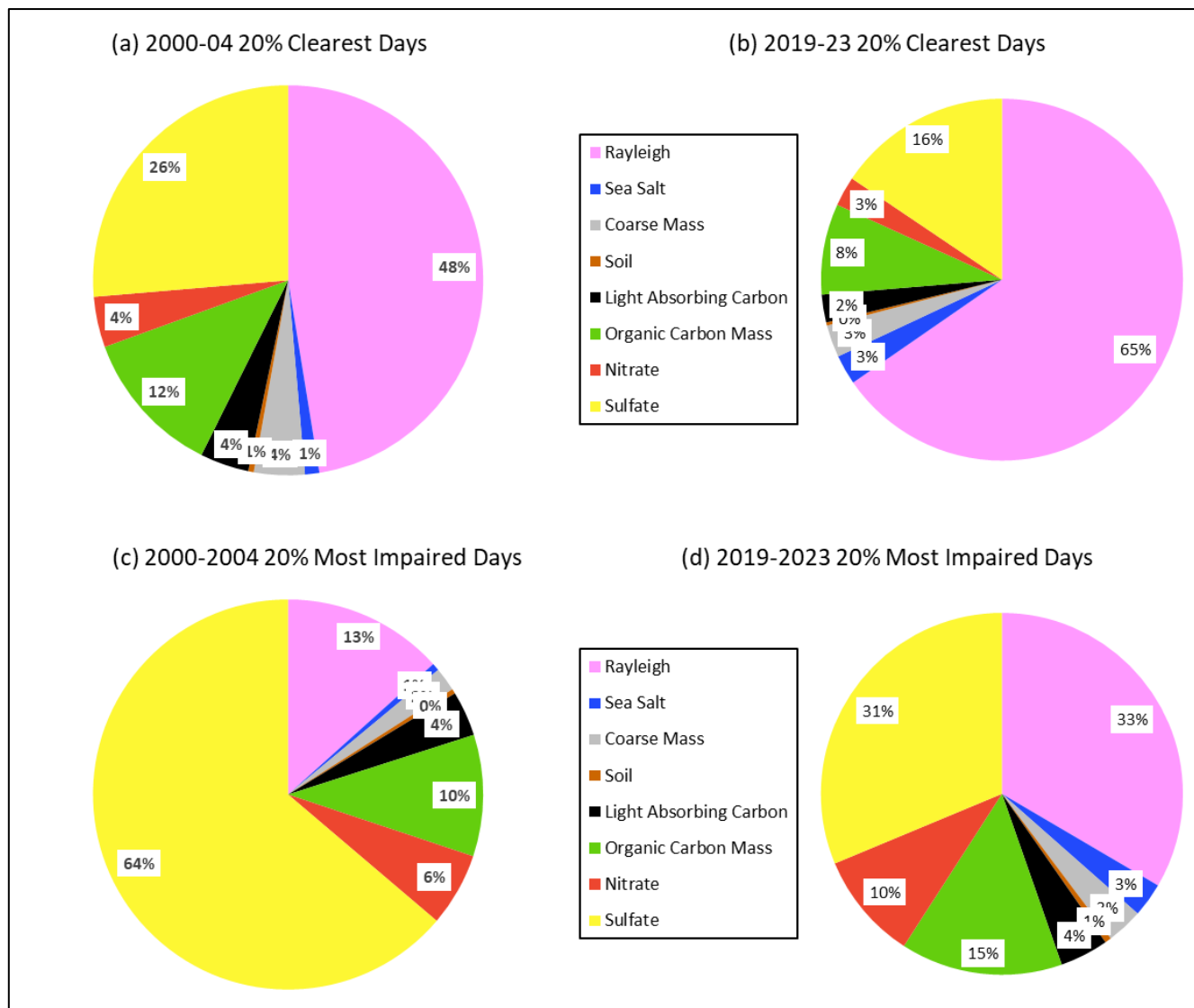
Figure 3-2. Moosehorn Wilderness Area Species Percent Contribution to Baseline (2000-04) and Current (2019-23) Haze Index Levels
