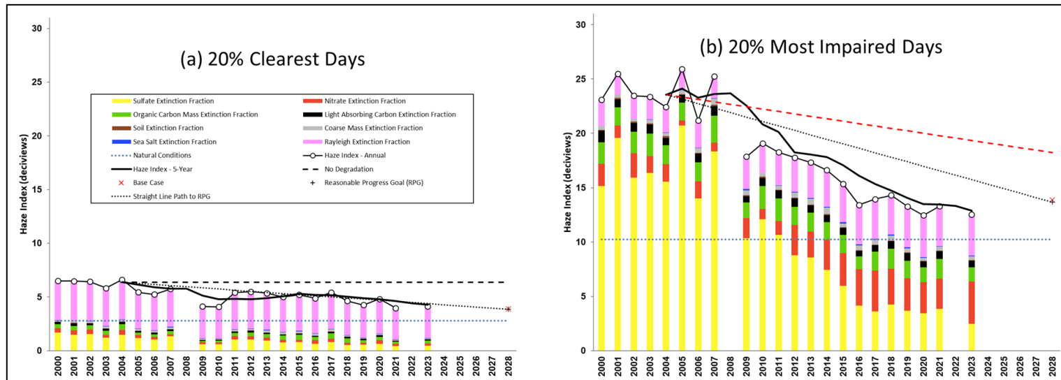
Figure 3-13. Individual Species Contribution to Annual Haze Index Levels at Lye Brook Wilderness Area on 20 Percent Clearest and Most Impaired Visibility Days
