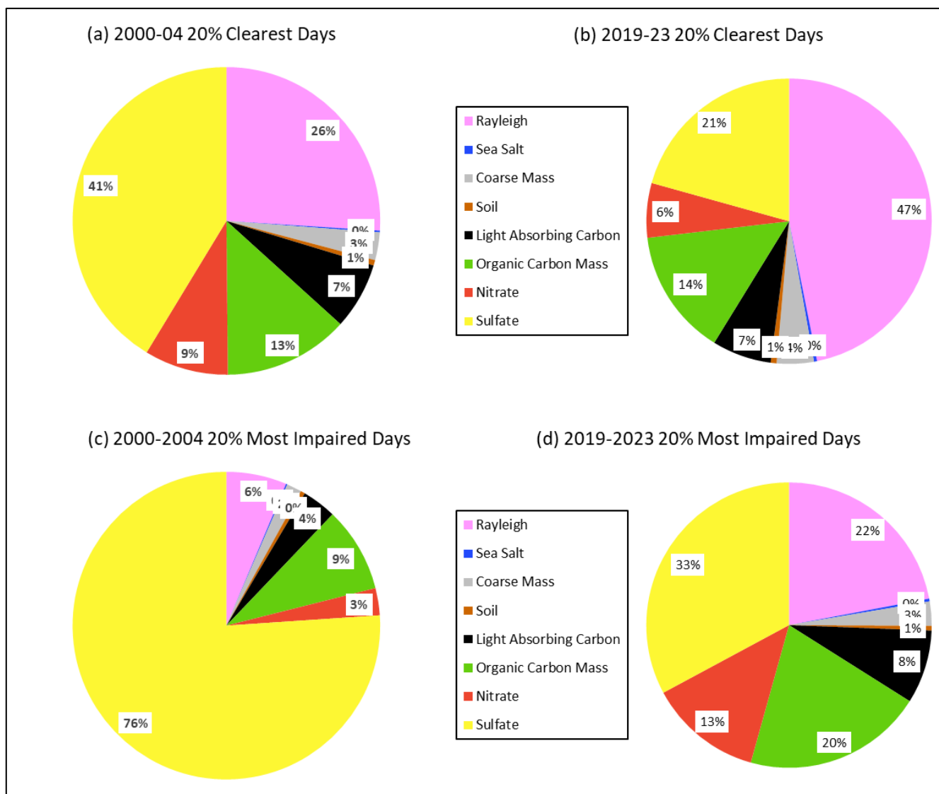
Figure 3-8. James River Face Wilderness Area Species Percent Contribution to Baseline (2000-04) and Current (2019-23) Haze Index Levels
