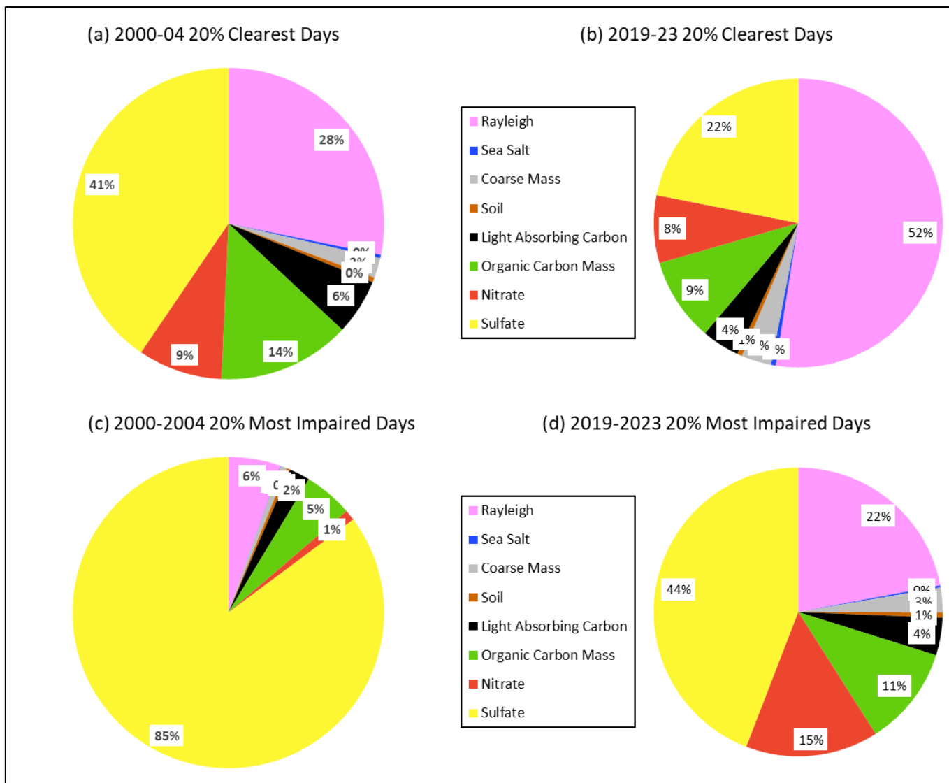
Figure 3-6. Dolly Sods Wilderness Area Species Percent Contribution to Baseline (2000-04) and Current (2019-23) Haze Index Levels
