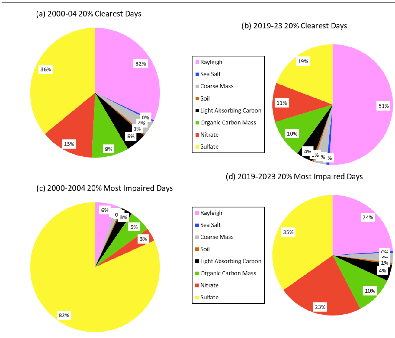
Figure 3-7. Shenandoah National Park Species Percent Contribution to Baseline (2000-04) and Current (2019-23) Haze Index Levels
