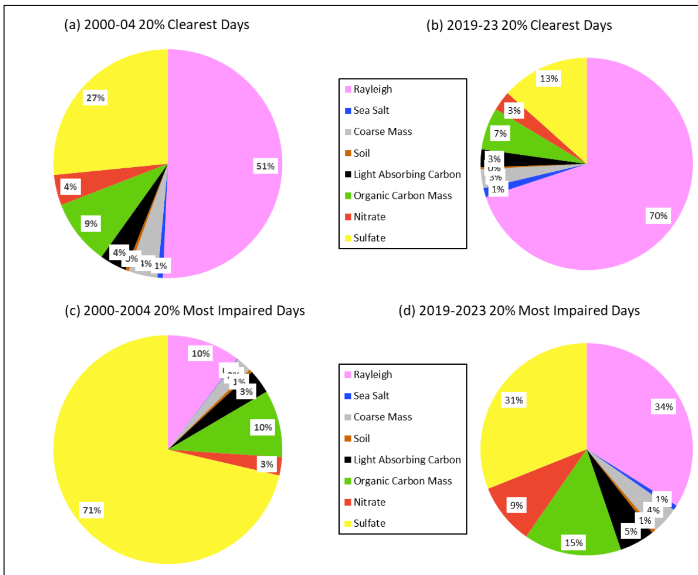
Figure 3-3. Great Gulf Wilderness Area Species Percent Contribution to Baseline (2000-04) and Current (2019-23) Haze Index Levels
