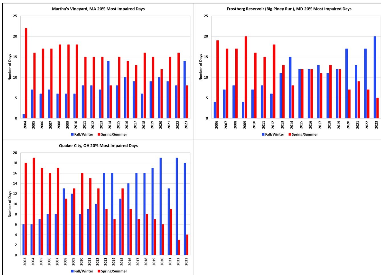
Figure C-3. Seasonal Breakdown of 20 Percent Most Impaired Visibility Days for Martha's Vineyard, MA, Maryland, and Ohio IMPROVE Protocol Sites
