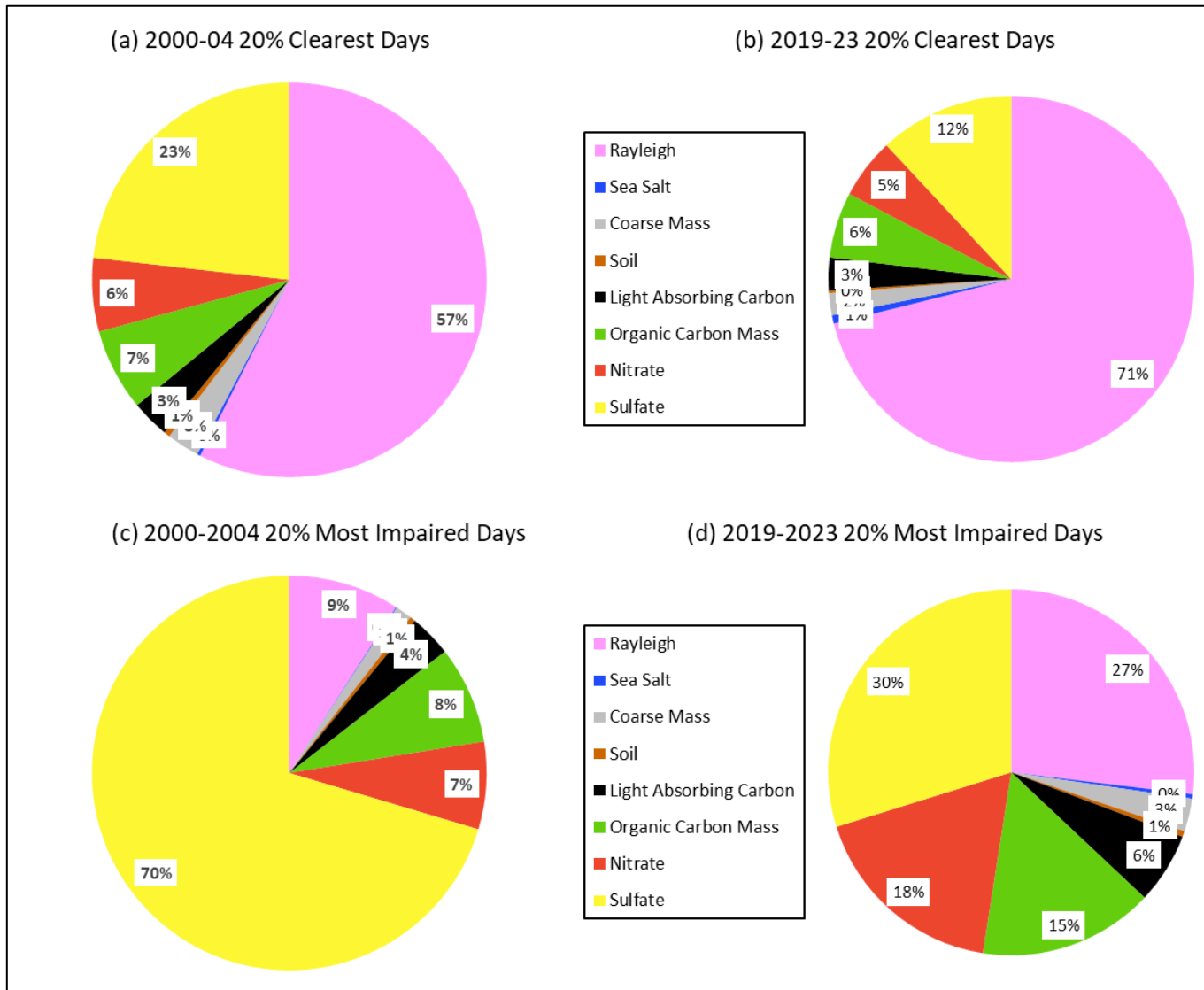
Figure 3-4. Lye Brook Wilderness Area Species Percent Contribution to Baseline (2000-04) and Current (2019-23) Haze Index Levels
