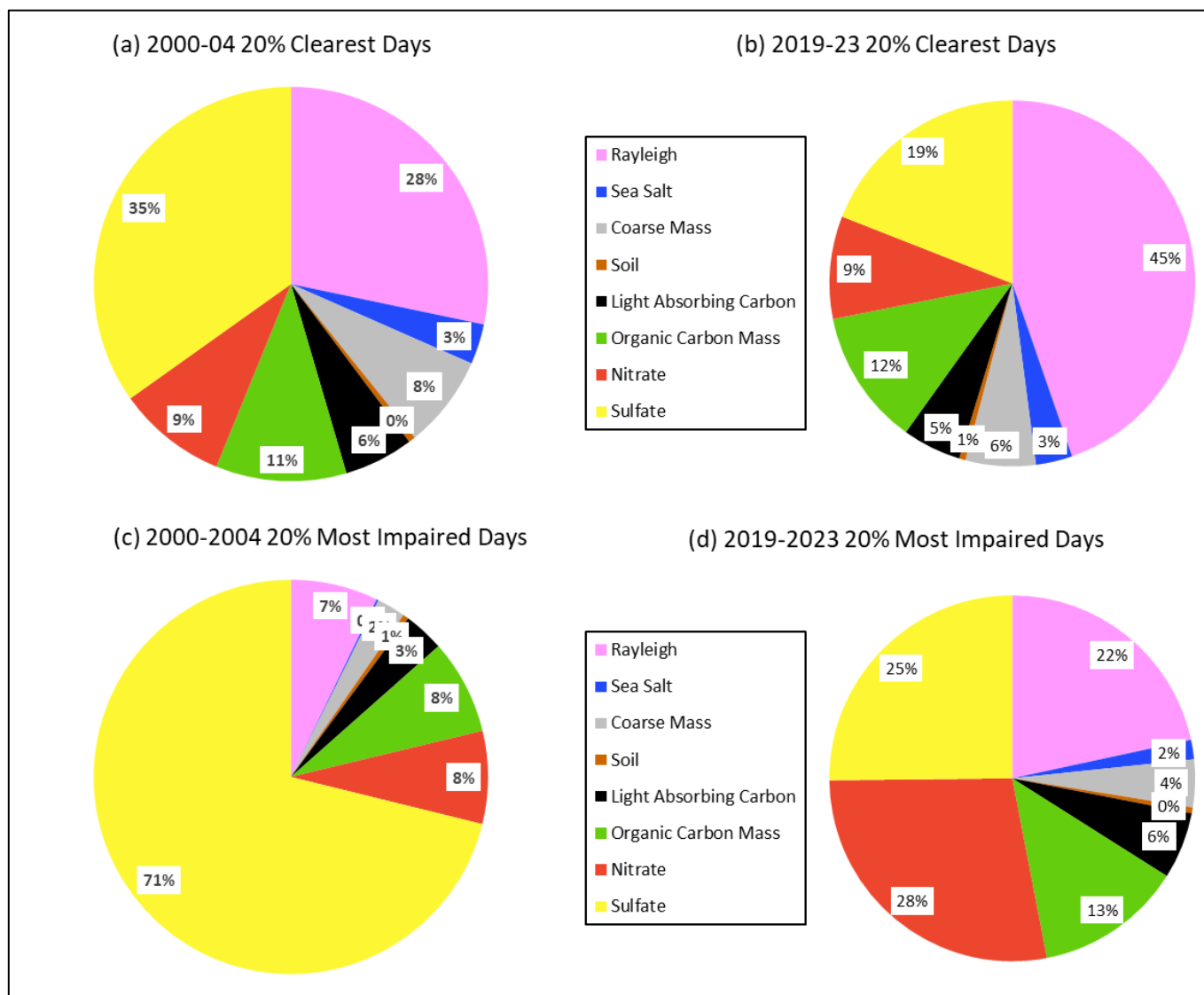
Figure 3-5. Brigantine Wilderness Area Species Percent Contribution to Baseline (2000-04) and Current (2019-23) Haze Index Levels
