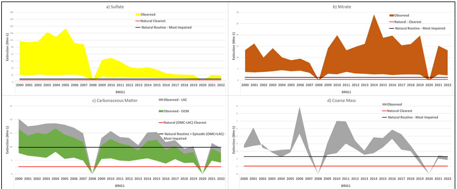
Figure D-5. Range of Observed and Estimated Natural Light Extinction for Select Individual Species at Brigantine on 20 Percent Clearest and Most Impaired Visibility Days
